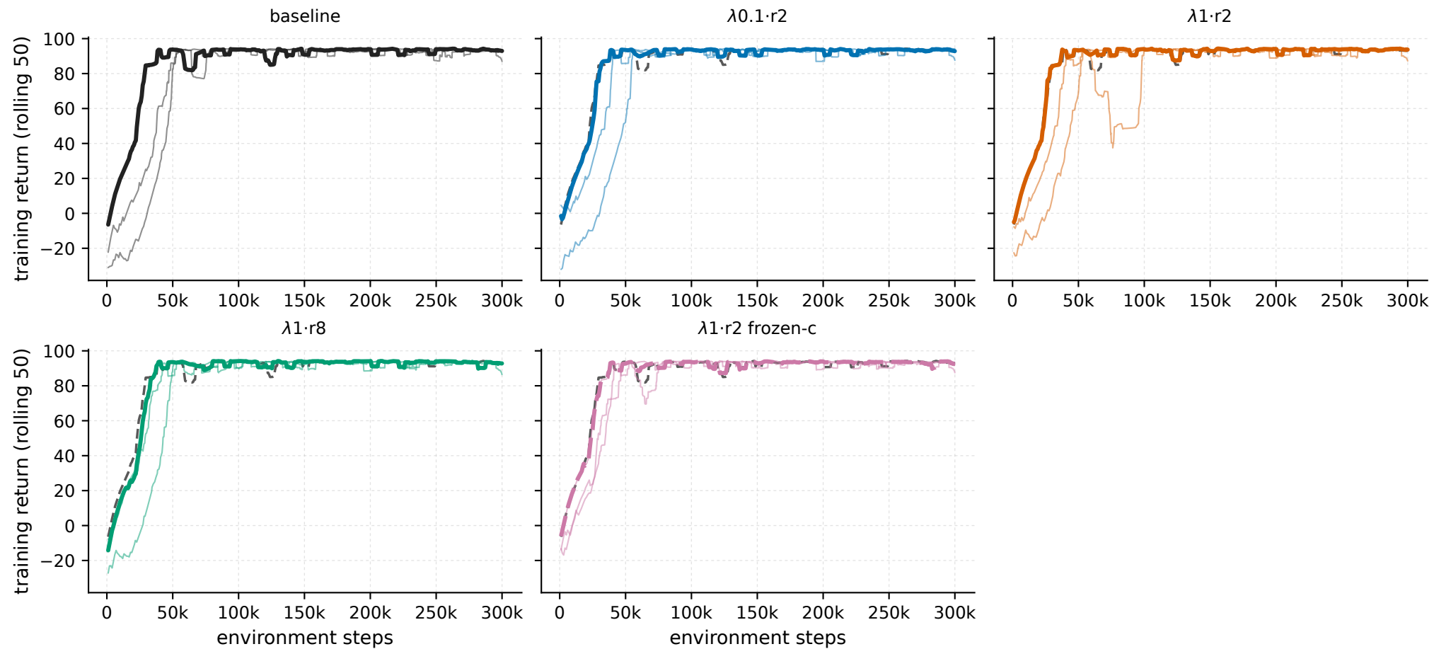
MountainCarContinuous-v0 - every seed per arm (train); grey dashed = baseline seed mean
