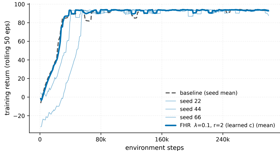
MountainCarContinuous-v0 - \lambda 0.1 \cdot r^2 , every seed (train)
