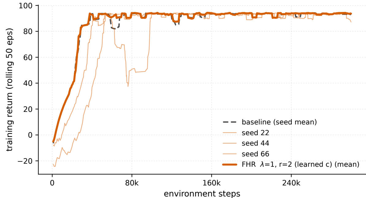
MountainCarContinuous-v0 - \lambda 1 \cdot r_2 , every seed (train)
