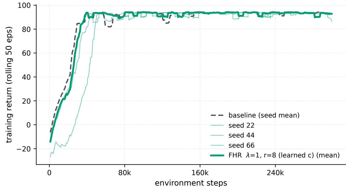
MountainCarContinuous-v0 - \lambda 1 \cdot r8 , every seed (train)
