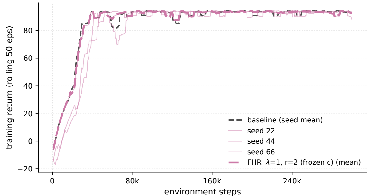
MountainCarContinuous-v0 - \lambda 1 \cdot r_2 frozen-c, every seed (train)
