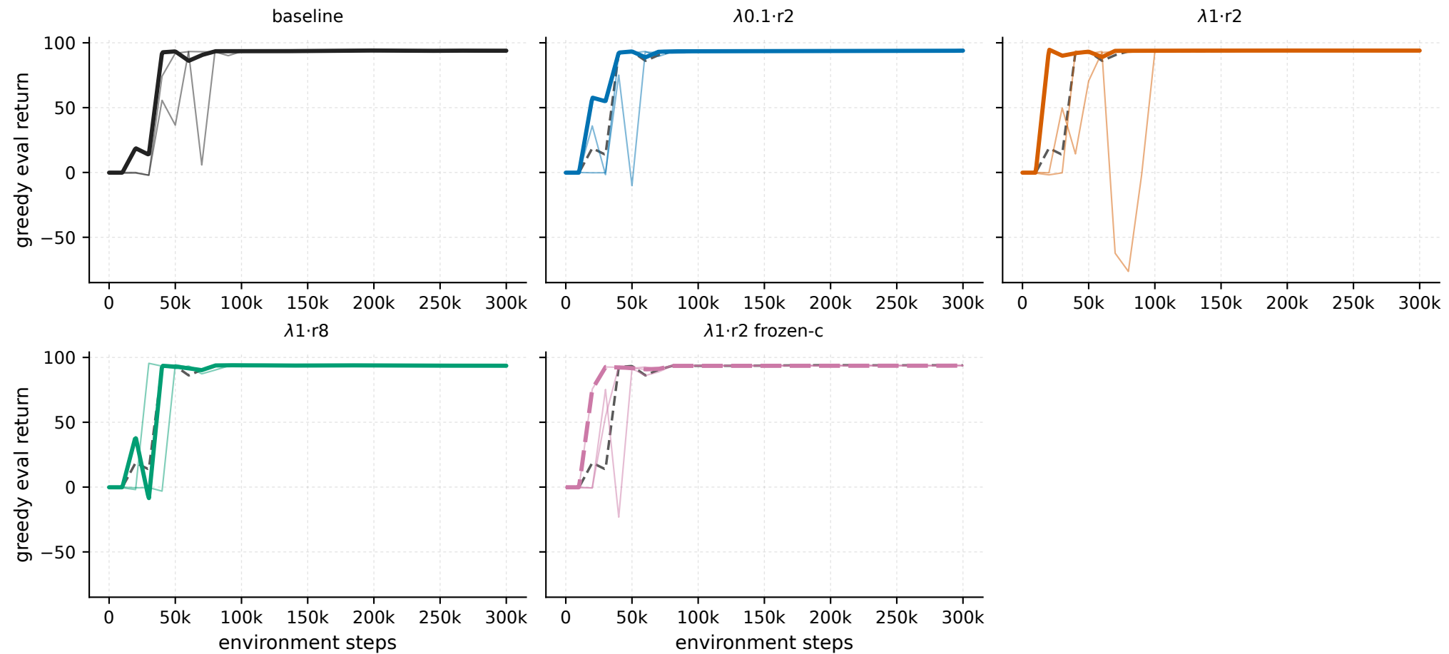
MountainCarContinuous-v0 - every seed per arm (eval); grey dashed = baseline seed mean
