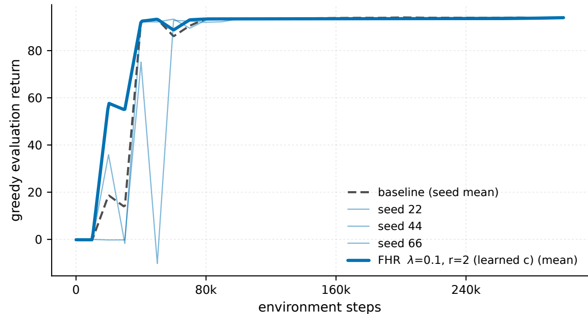
MountainCarContinuous-v0 - \lambda 0.1 \cdot r_2 , every seed (eval)
