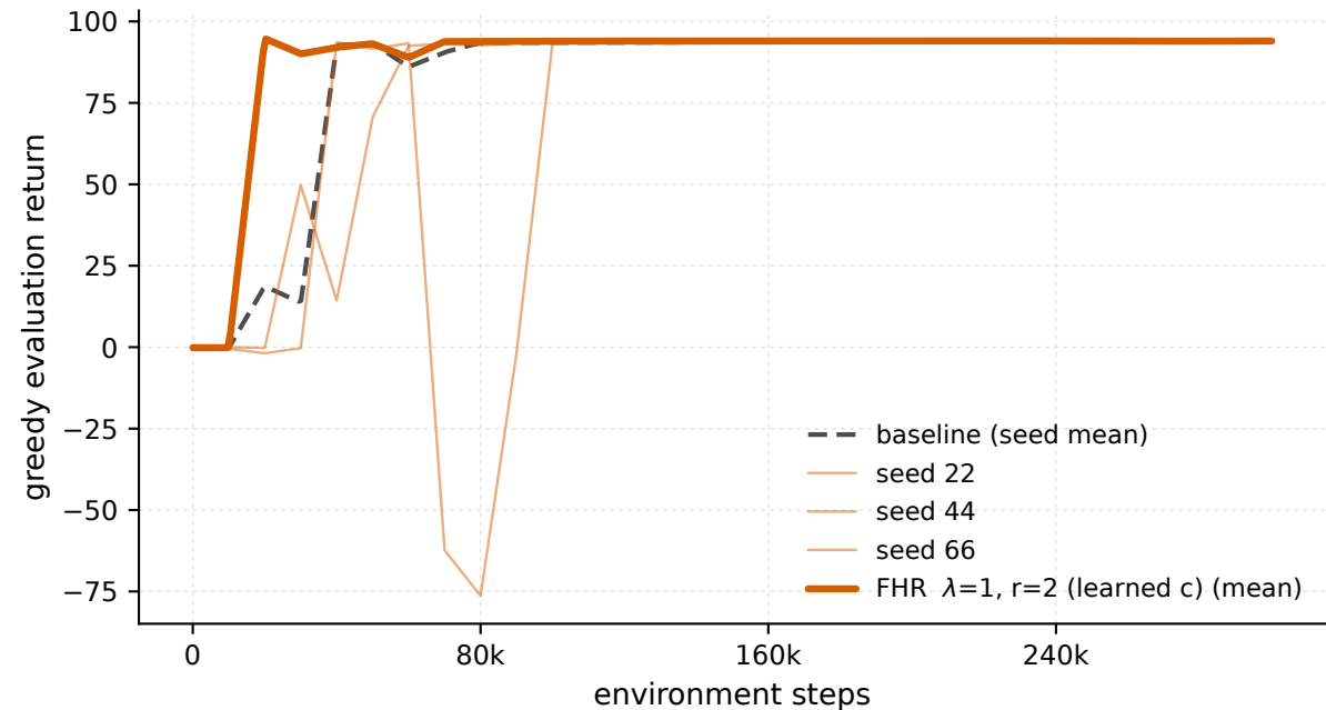
MountainCarContinuous-v0 - \lambda 1 \cdot r_2 , every seed (eval)
