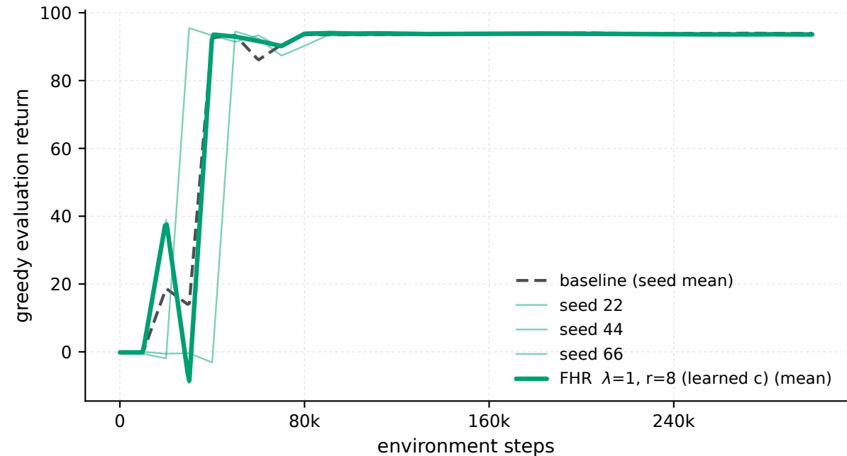
MountainCarContinuous-v0 - \lambda 1 \cdot r8 , every seed (eval)
