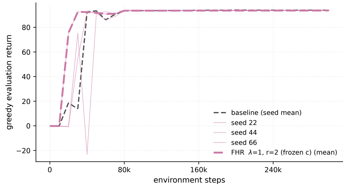
MountainCarContinuous-v0 - \lambda 1 \cdot r 2 frozen-c, every seed (eval)
