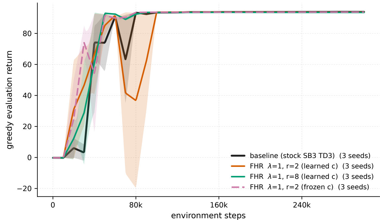
MountainCarContinuous-v0 - lambda = 1: learned vs frozen-theory c (eval)
