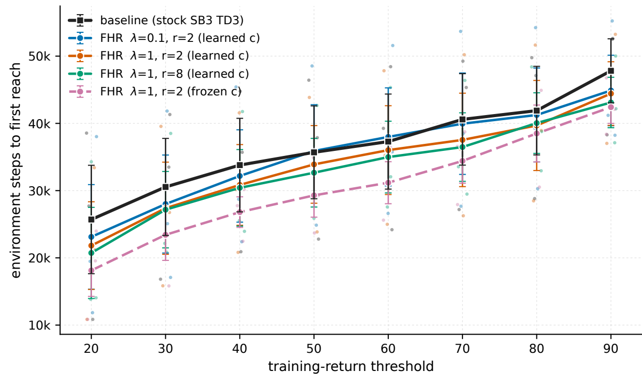
MountainCarContinuous-v0 - sample efficiency, training stream (mean \pm 1 s.e.m.)
