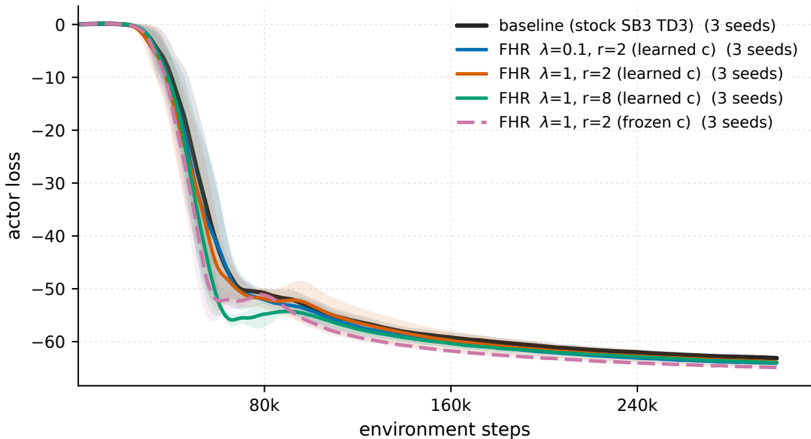
MountainCarContinuous-v0 - actor loss
