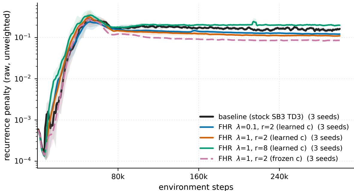
MountainCarContinuous-v0 - recurrence penalty (raw, unweighted)
