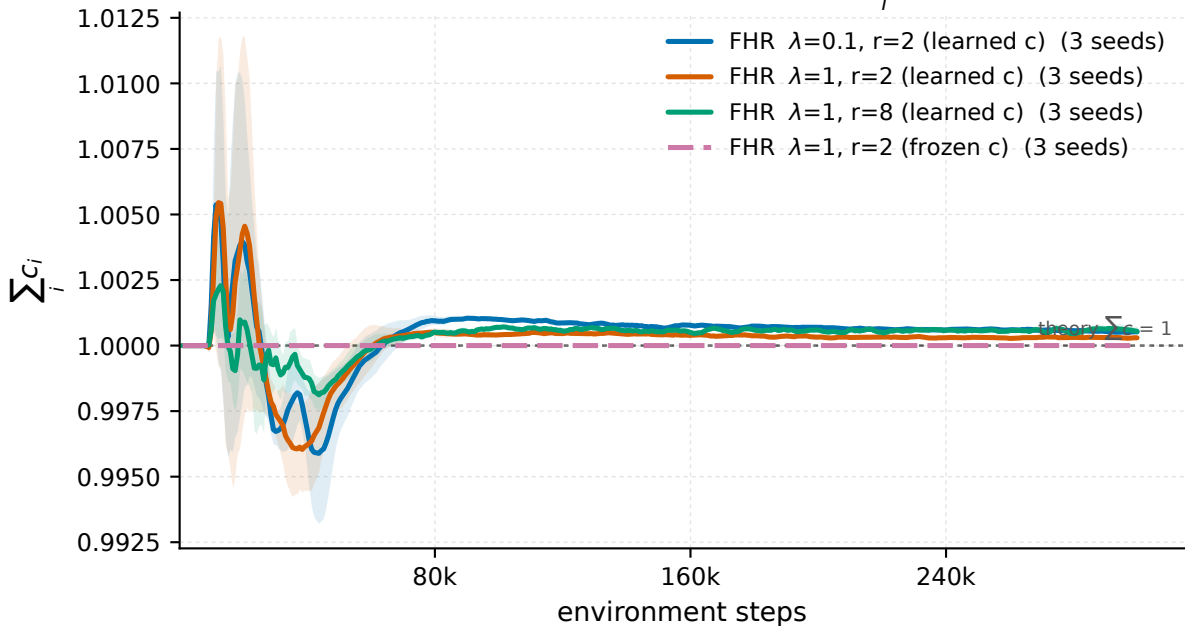
MountainCarContinuous-v0 - \sum_i c_i
