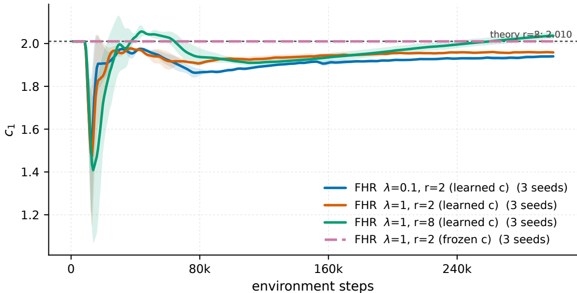
MountainCarContinuous-v0 - recurrence coefficient c_1 vs the Bellman theory value
