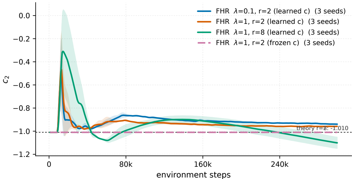
MountainCarContinuous-v0 - recurrence coefficient c_2 vs the Bellman theory value
