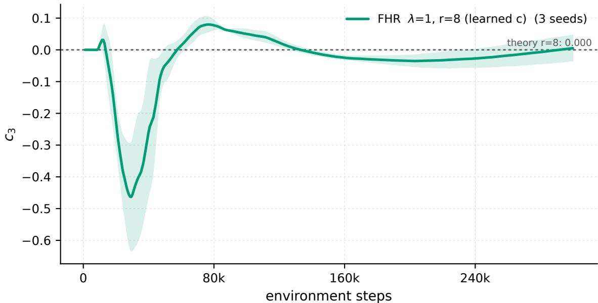
MountainCarContinuous-v0 - recurrence coefficient c_3 vs the Bellman theory value
