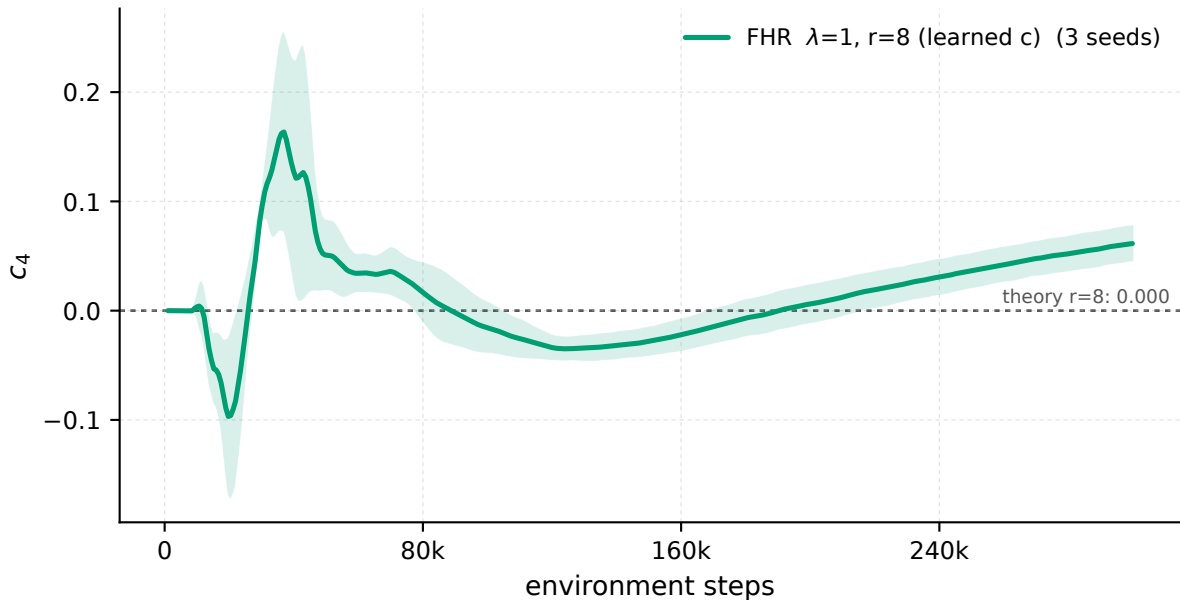
MountainCarContinuous-v0 - recurrence coefficient c_4 vs the Bellman theory value
