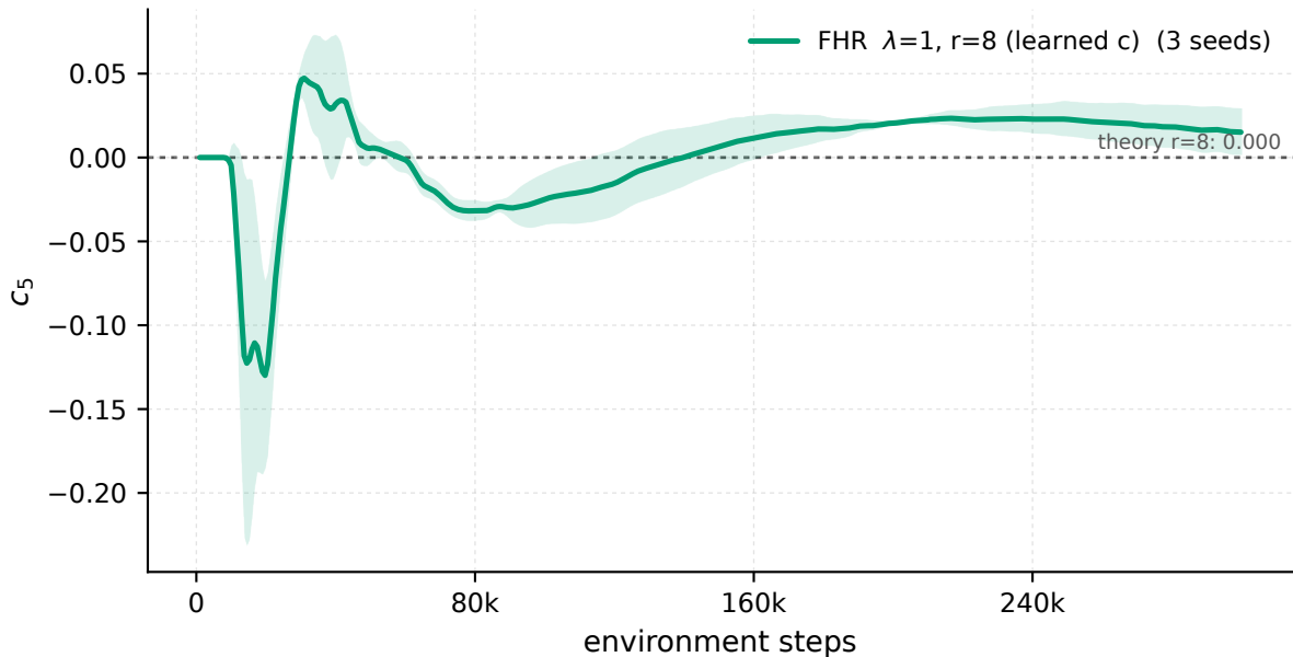
MountainCarContinuous-v0 - recurrence coefficient c_5 vs the Bellman theory value
