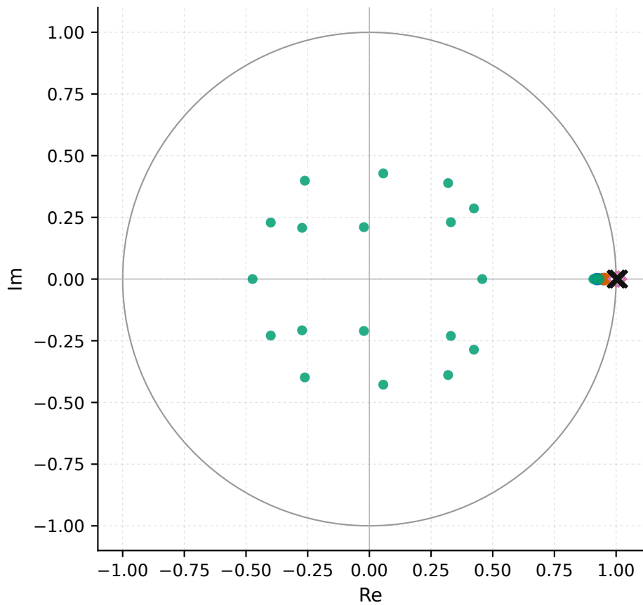
MountainCarContinuous-v0 - companion roots of the learned recurrence (final, per seed)
