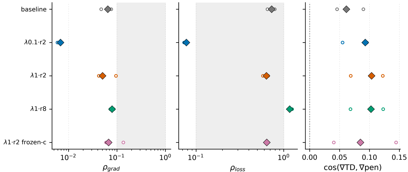
MountainCarContinuous-v0 - stream ratios, tail medians over the last 50% (baseline: unweighted); shaded = target range
