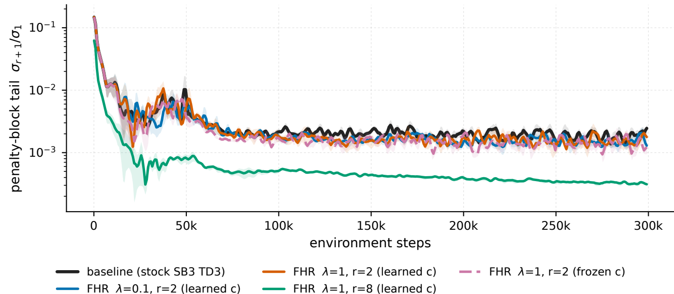
MountainCarContinuous-v0 - penalised windows, all arms penalty-block tail \sigma_{r+1}/\sigma_1
