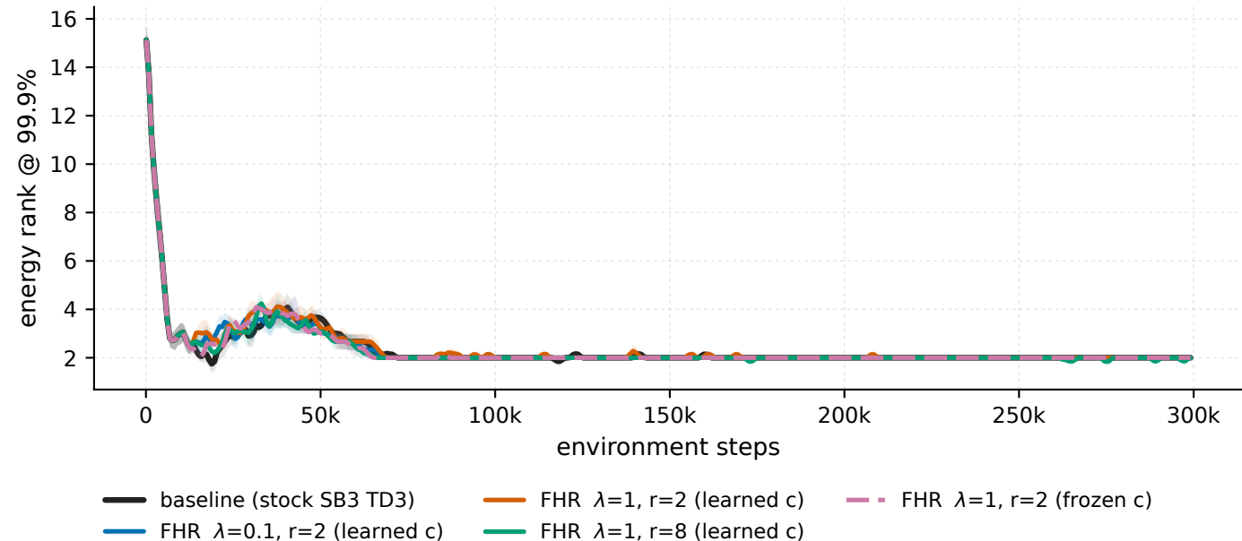
MountainCarContinuous-v0 - penalised windows, all arms energy rank @ 99.9%
