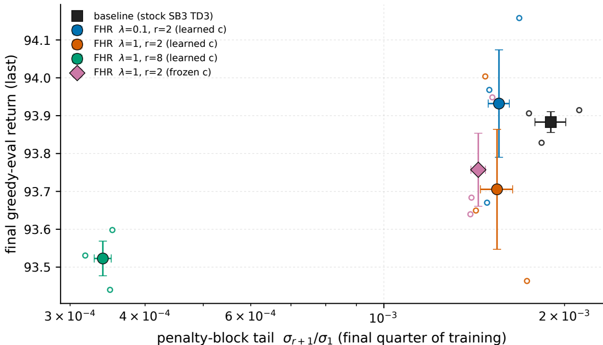
MountainCarContinuous-v0 - penalised-window compression vs return
