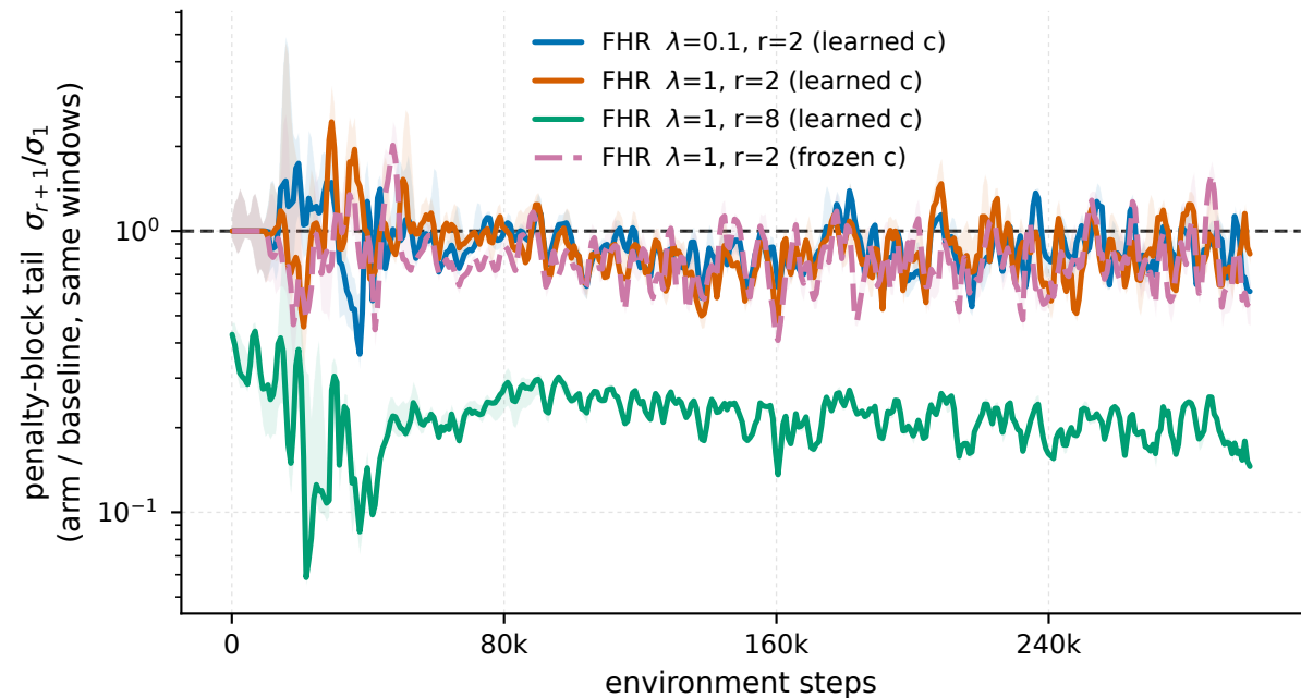
MountainCarContinuous-v0 - compression relative to the baseline
