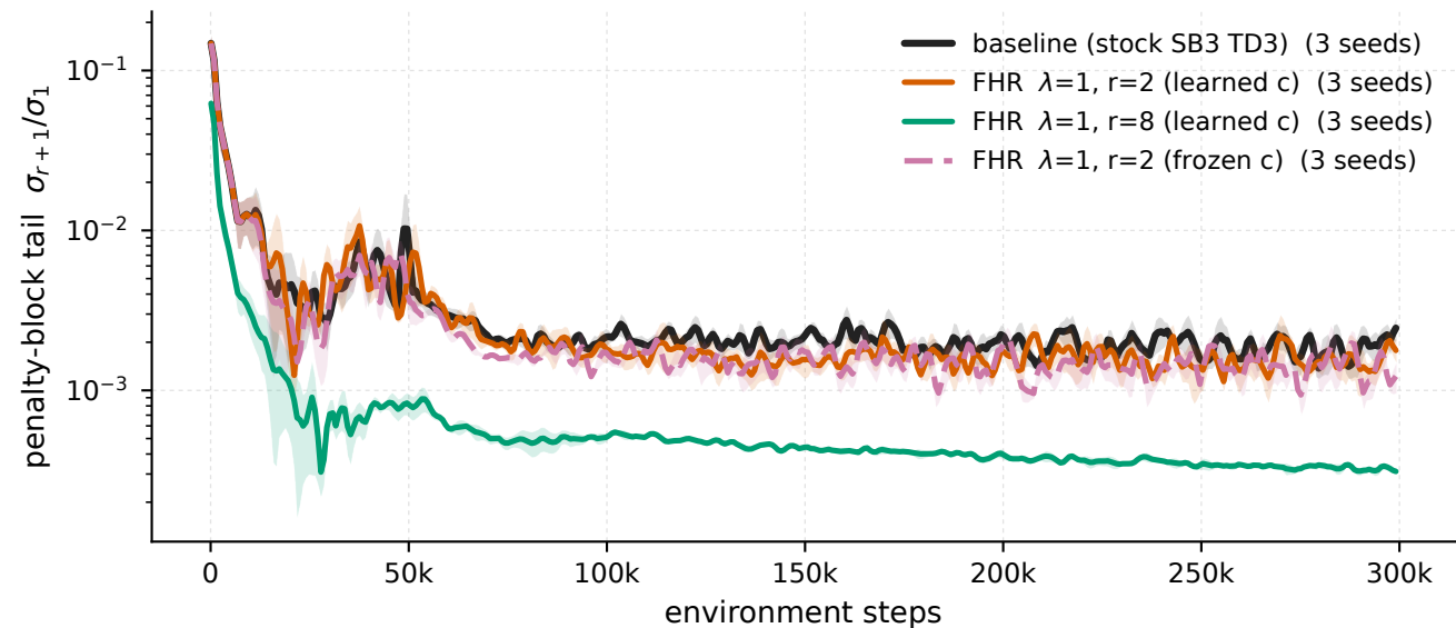
MountainCarContinuous-v0 - \lambda 1 \cdot r_2 , \lambda 1 \cdot r_8 , \lambda 1 \cdot r_2 frozen-c vs baseline, penalised windows penalty-block tail \sigma_{r+1}/\sigma_1
