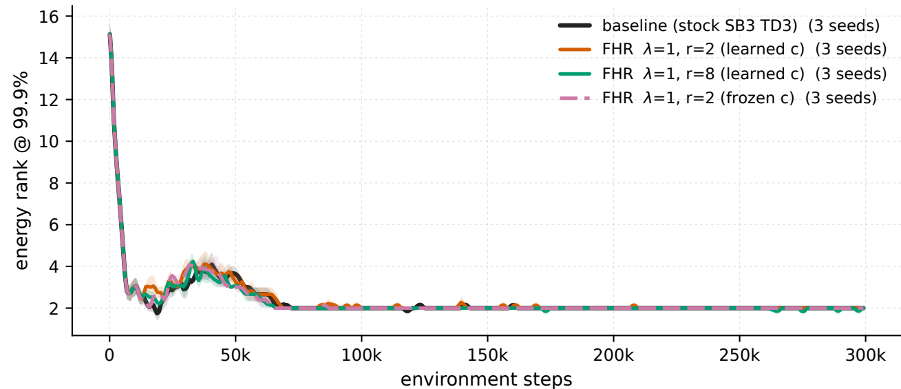
MountainCarContinuous-v0 - \lambda 1 \cdot r_2 , \lambda 1 \cdot r_8 , \lambda 1 \cdot r_2 frozen-c vs baseline, penalised windows energy rank @ 99.9%
