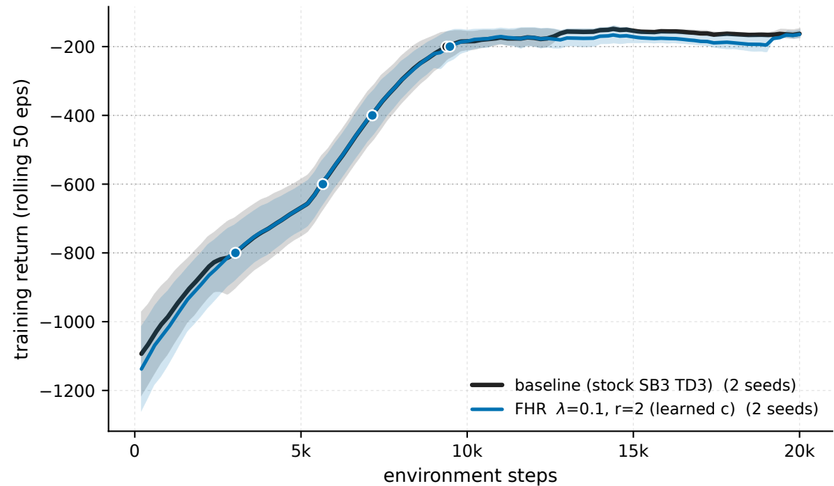
Pendulum-v1 - \lambda 0.1 \cdot r_2 vs baseline (training stream)
