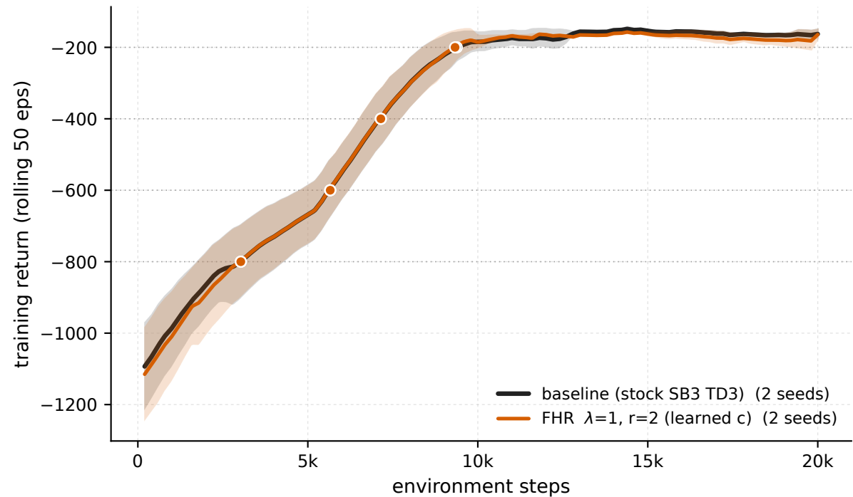
Pendulum-v1 - \lambda 1 \cdot r_2 vs baseline (training stream)
