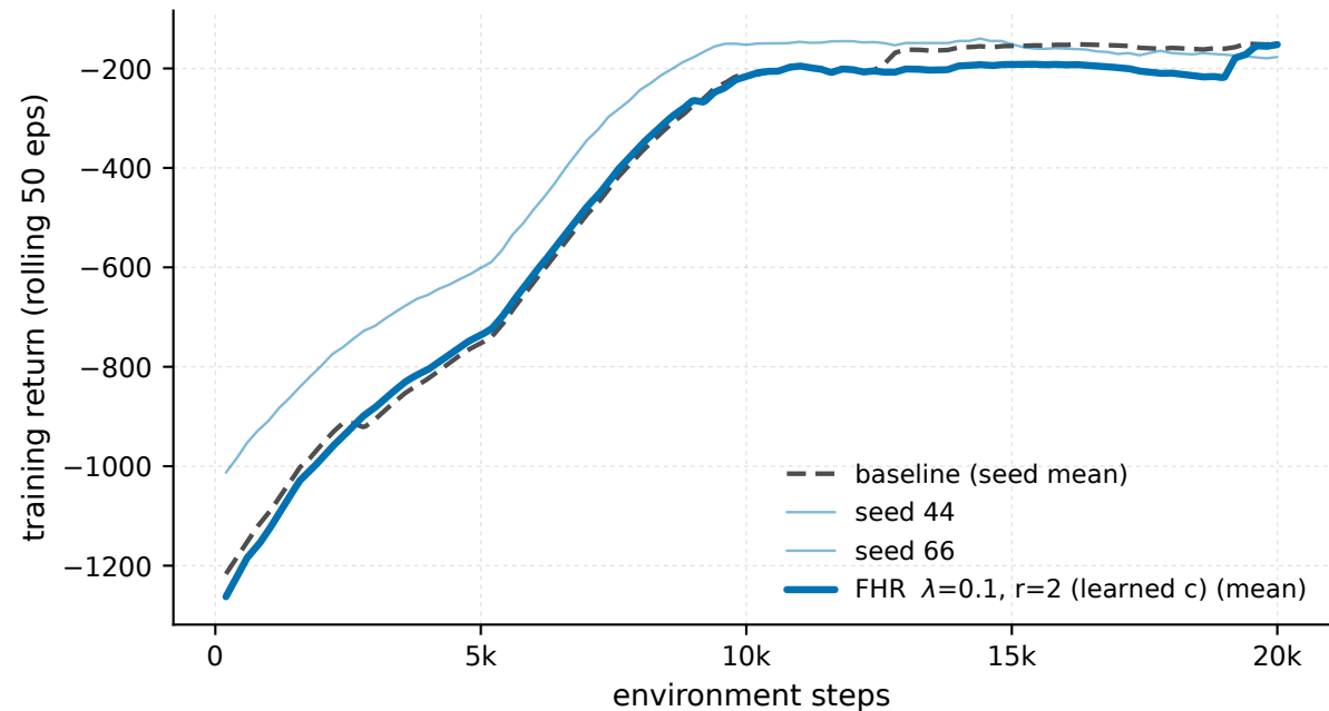
Pendulum-v1 - \lambda 0.1 \cdot r_2 , every seed (train)
