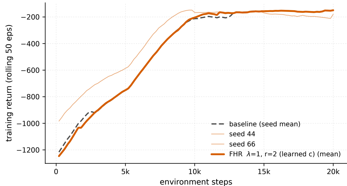
Pendulum-v1 - \lambda 1 \cdot r_2 , every seed (train)
