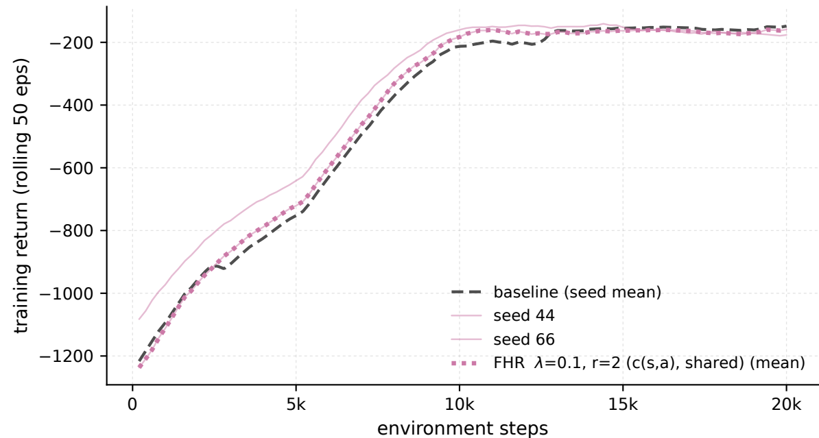
Pendulum-v1 - \lambda 0.1 \cdot r_2 c(s,a) shared, every seed (train)
