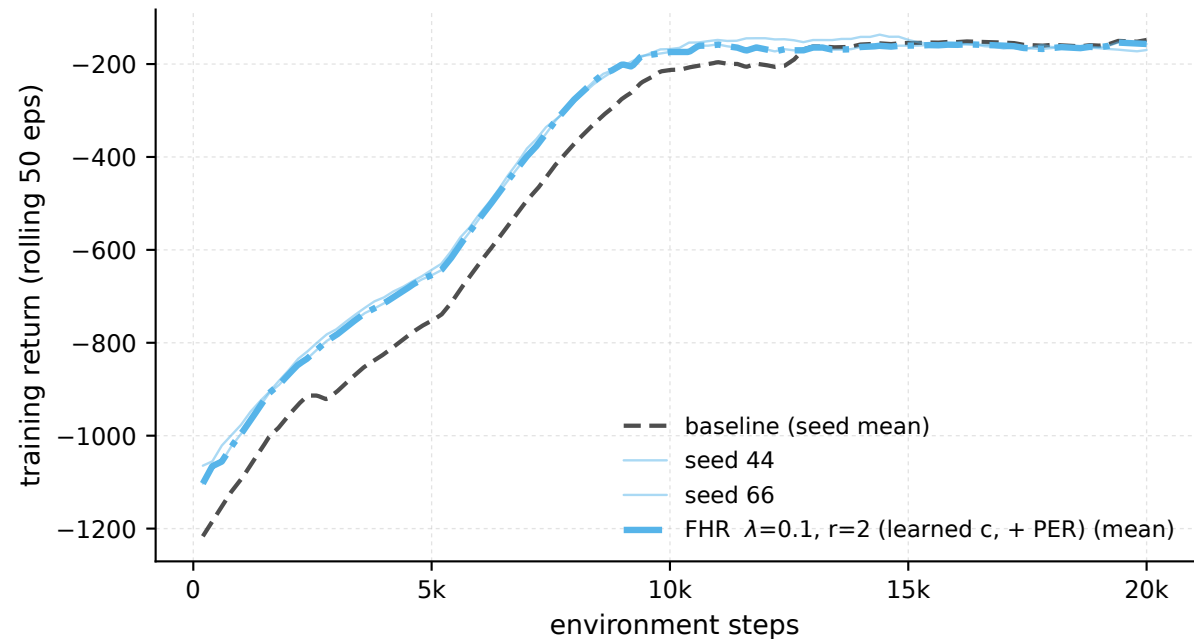
Pendulum-v1 - \lambda 0.1 \cdot r_2 +PER, every seed (train)
