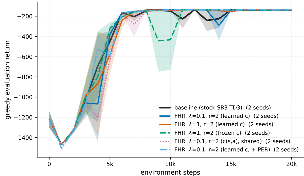
Pendulum-v1 - all arms (eval)
