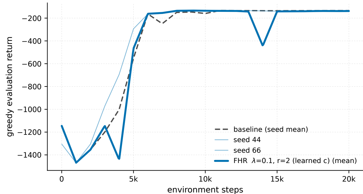
Pendulum-v1 - \lambda 0.1 \cdot r_2 , every seed (eval)
