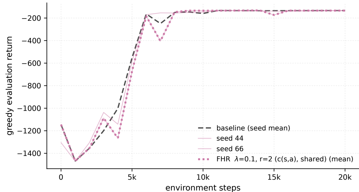
Pendulum-v1 - \lambda 0.1 \cdot r_2 c(s,a) shared, every seed (eval)
