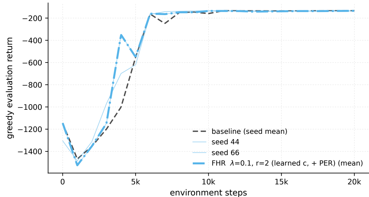
Pendulum-v1 - \lambda 0.1 \cdot r_2 +PER, every seed (eval)
