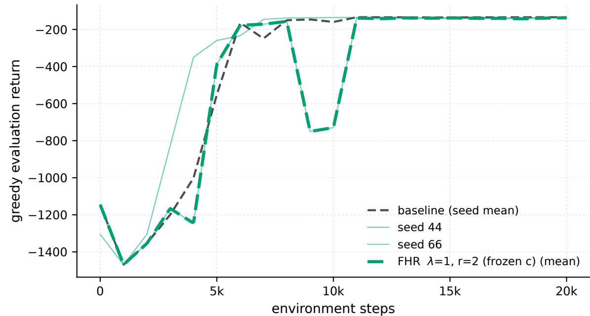
Pendulum-v1 - \lambda 1 \cdot r2 frozen-c, every seed (eval)
