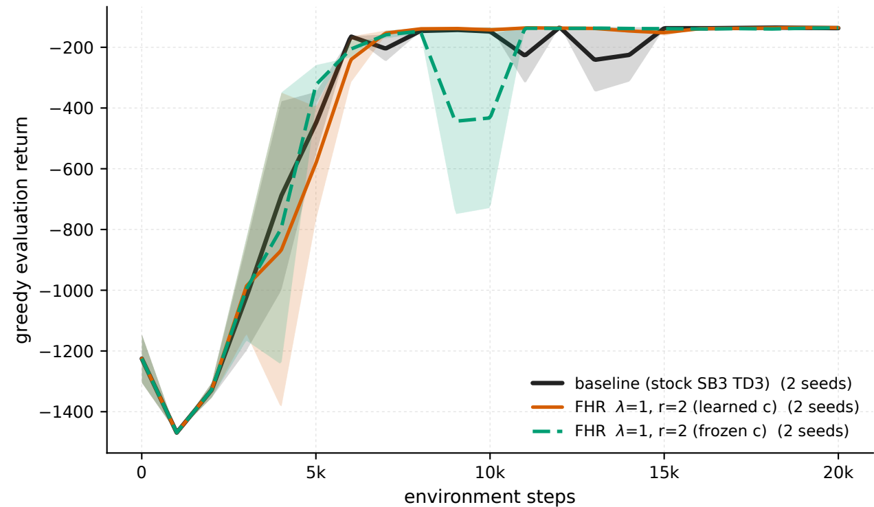
Pendulum-v1 - lambda = 1: learned vs frozen-theory c (eval)
