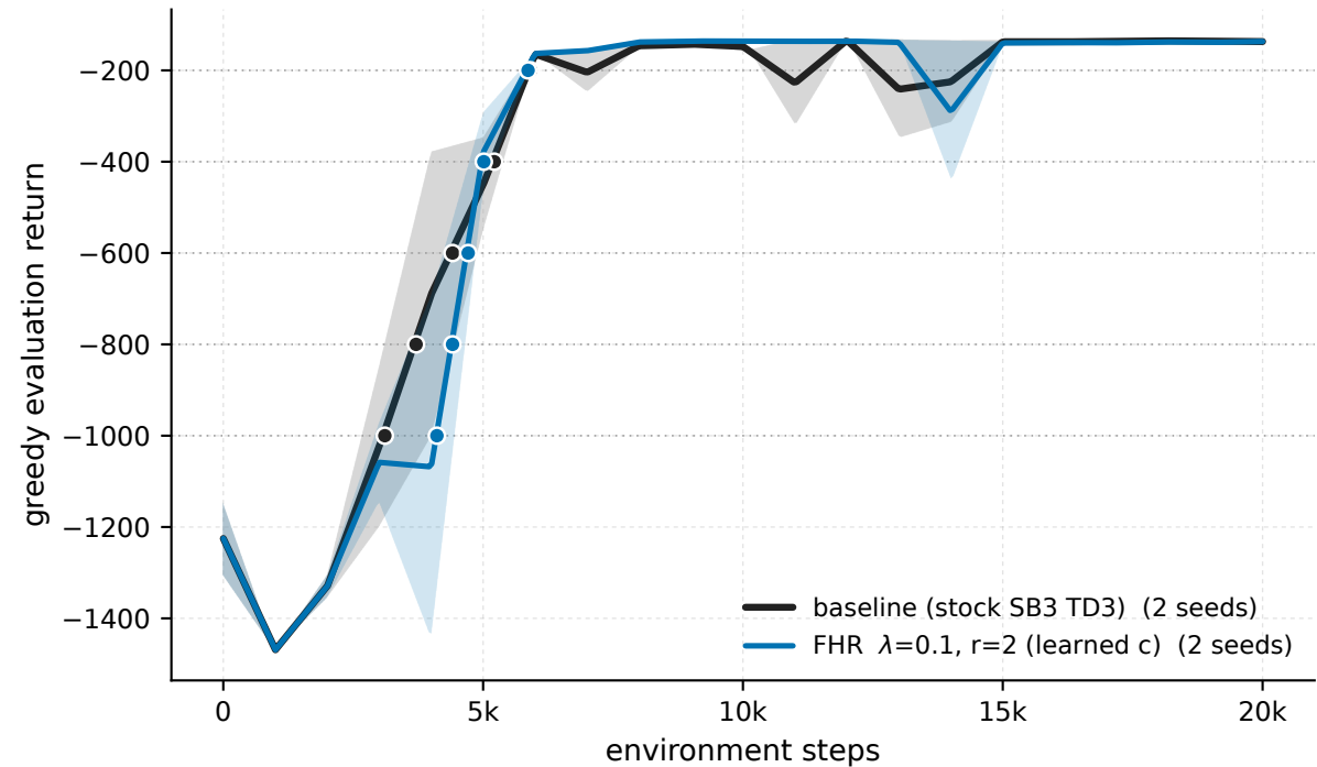
Pendulum-v1 - \lambda 0.1 \cdot r_2 vs baseline (greedy eval)
