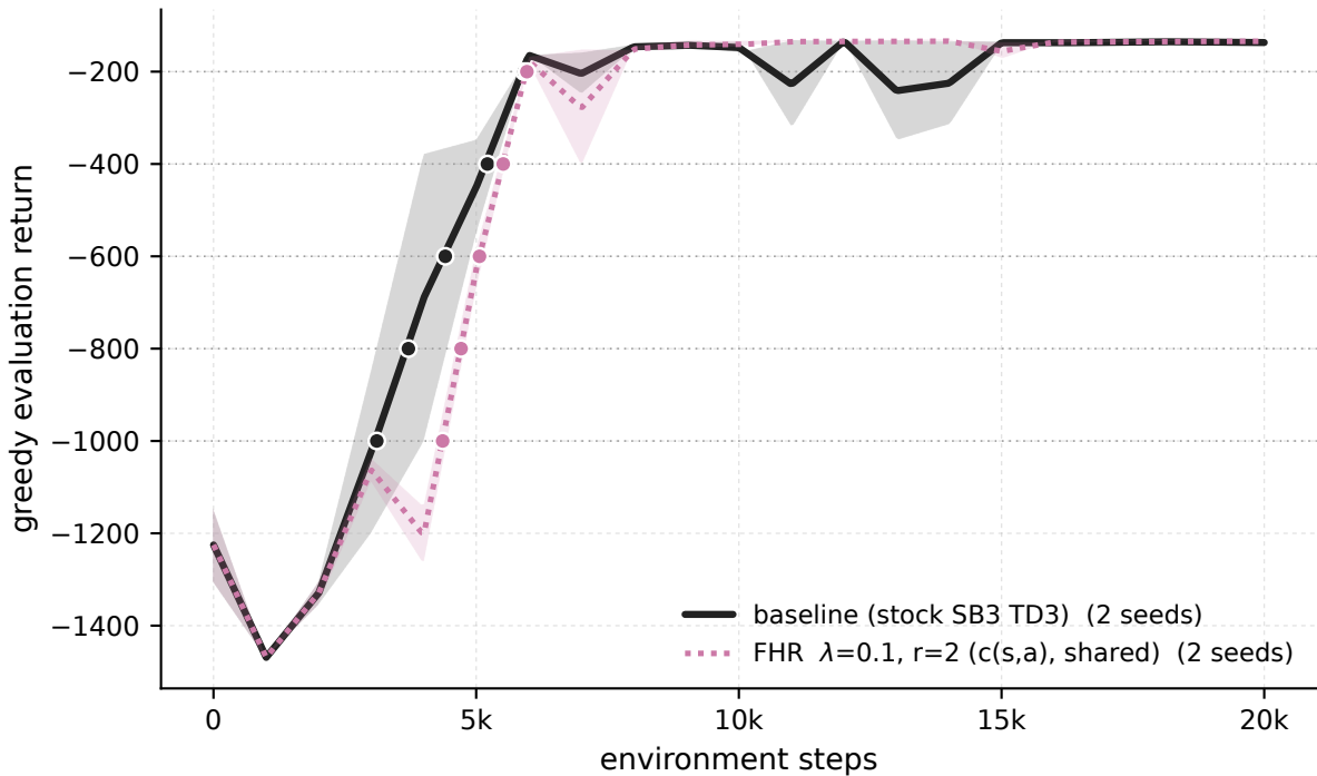
Pendulum-v1 - \lambda 0.1 \cdot r_2 c(s,a) shared vs baseline (greedy eval)
