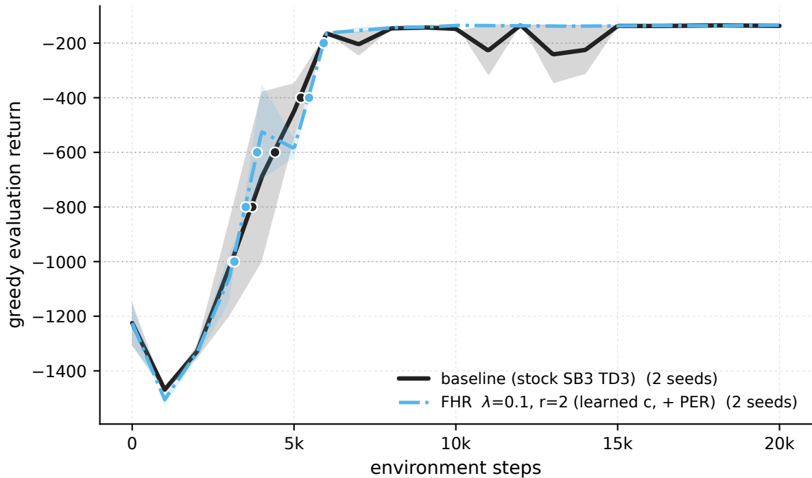
Pendulum-v1 - \lambda 0.1 \cdot r_2 +PER vs baseline (greedy eval)
