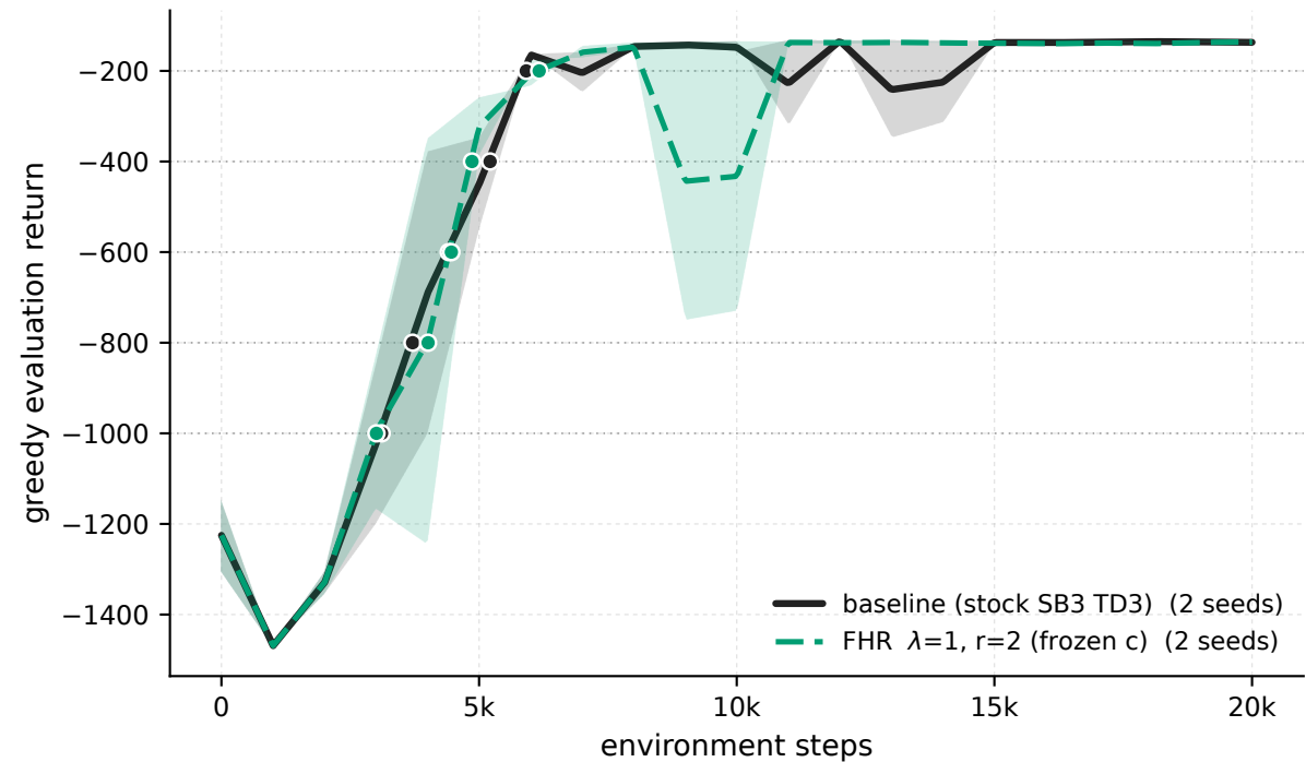
Pendulum-v1 - \lambda 1 \cdot r2 frozen-c vs baseline (greedy eval)
