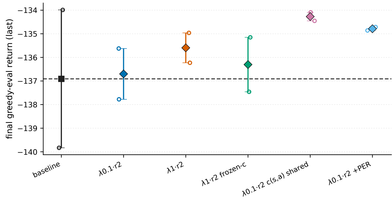
Pendulum-v1 - final return per arm: seeds (o), IQM with 95% bootstrap CI; dashed = baseline IQM
