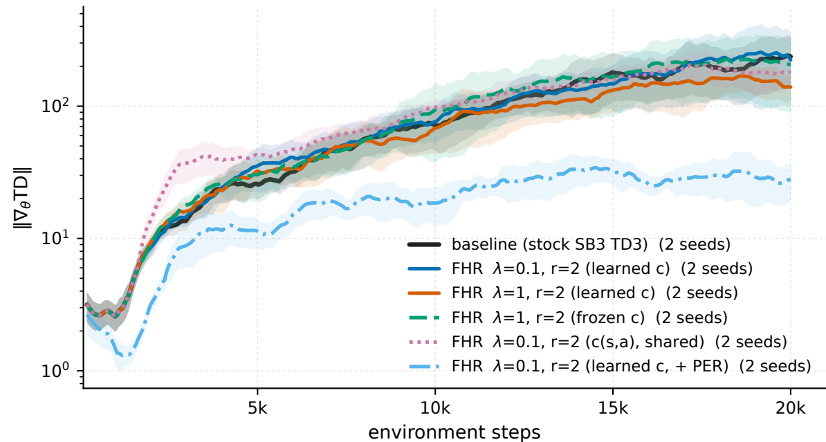
Pendulum-v1 - \|\nabla_{\theta}TD\|
