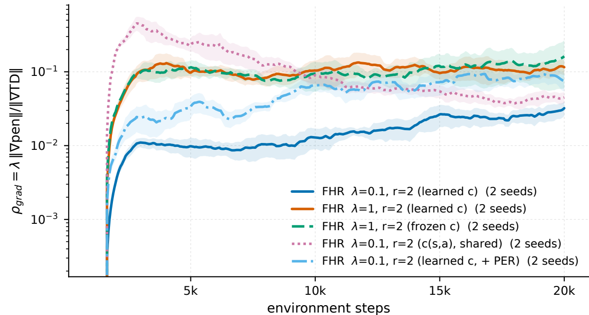
Pendulum-v1 - \rho_{grad} = \lambda \|\nabla pen\|/\|\nabla TD\|
