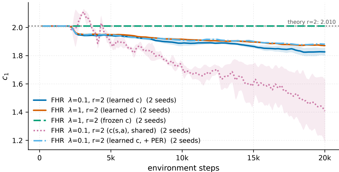
Pendulum-v1 - recurrence coefficient c_1 vs the Bellman theory value
