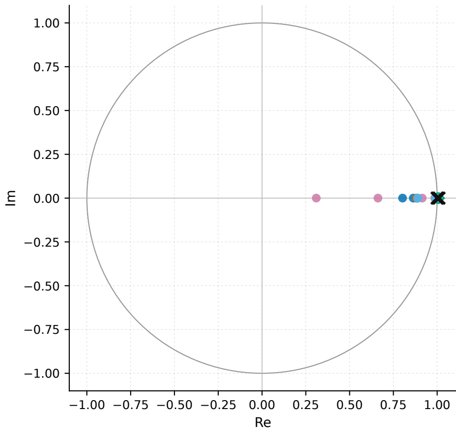
Pendulum-v1 - companion roots of the learned recurrence (final, per seed)
