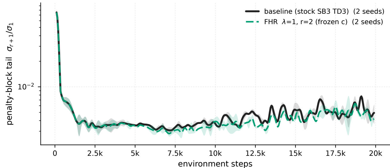
Pendulum-v1 - \lambda 1 \cdot r_2 frozen-c vs baseline, penalised windows penalty-block tail \sigma_{r+1}/\sigma_1
